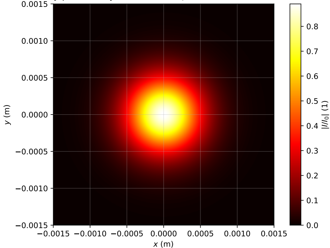
Intensity profile I(x, y, z = 1.433m)/I_0 , P_{in}=0.4P_{cr} , artificial time
